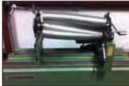
Roots Blower Scroll Precision Balancing
