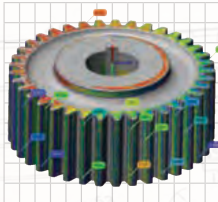
Dimensional Overlay of OEM vs. PowerRail Gear
