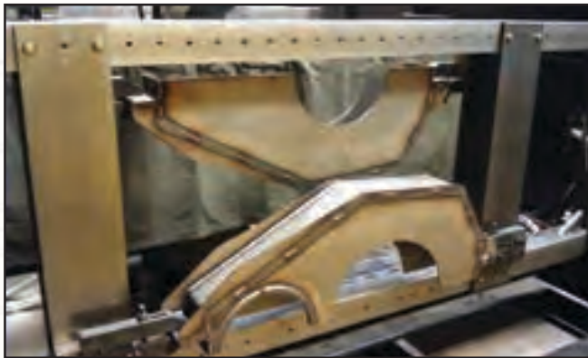
Latest Technology Robotic Fixture - Dual Sides
