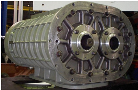
Right & Left Hand Roots Blowers
